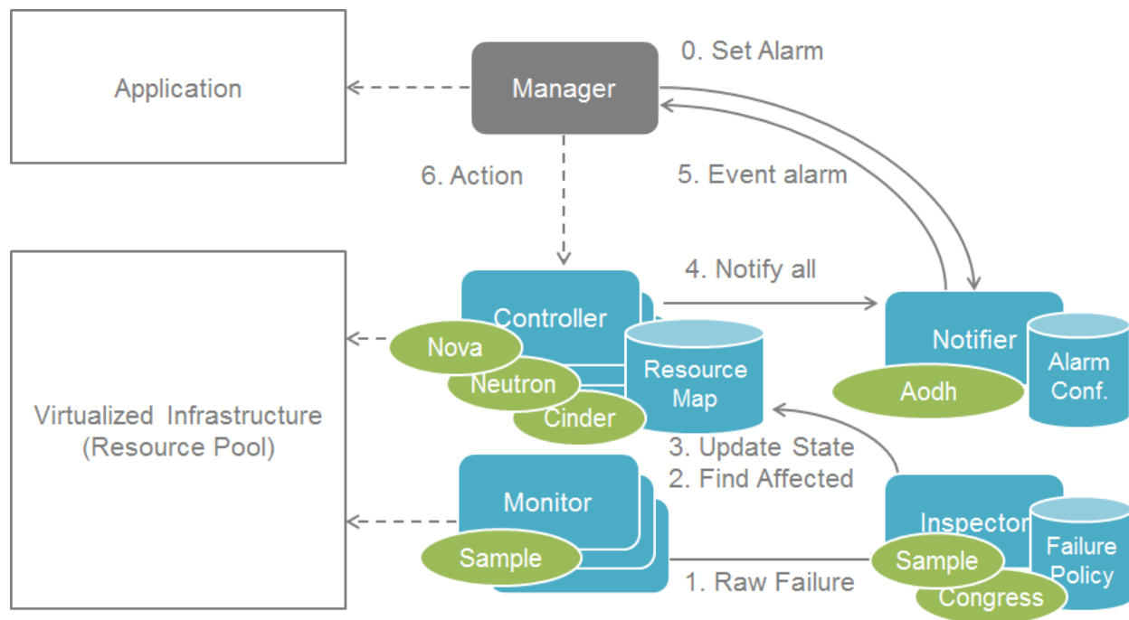
Fig. 1: Conservative Notification
