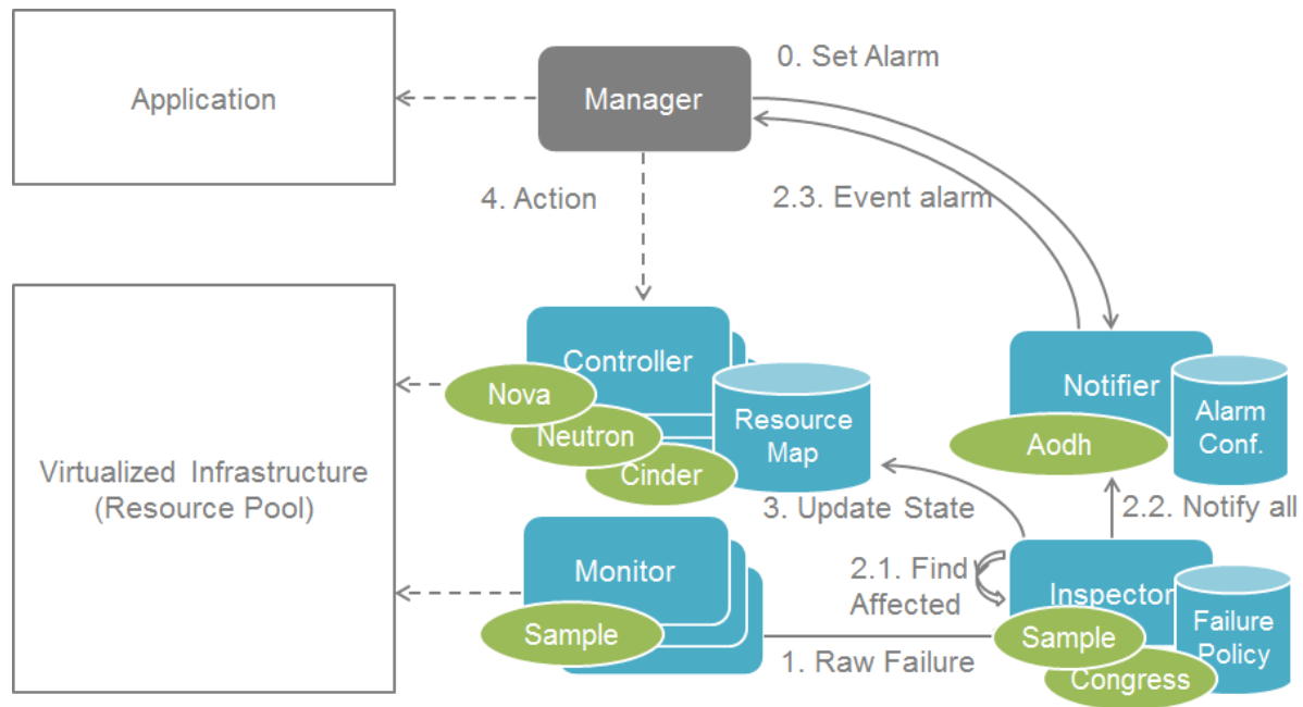
Fig. 2: Shortcut Notification
