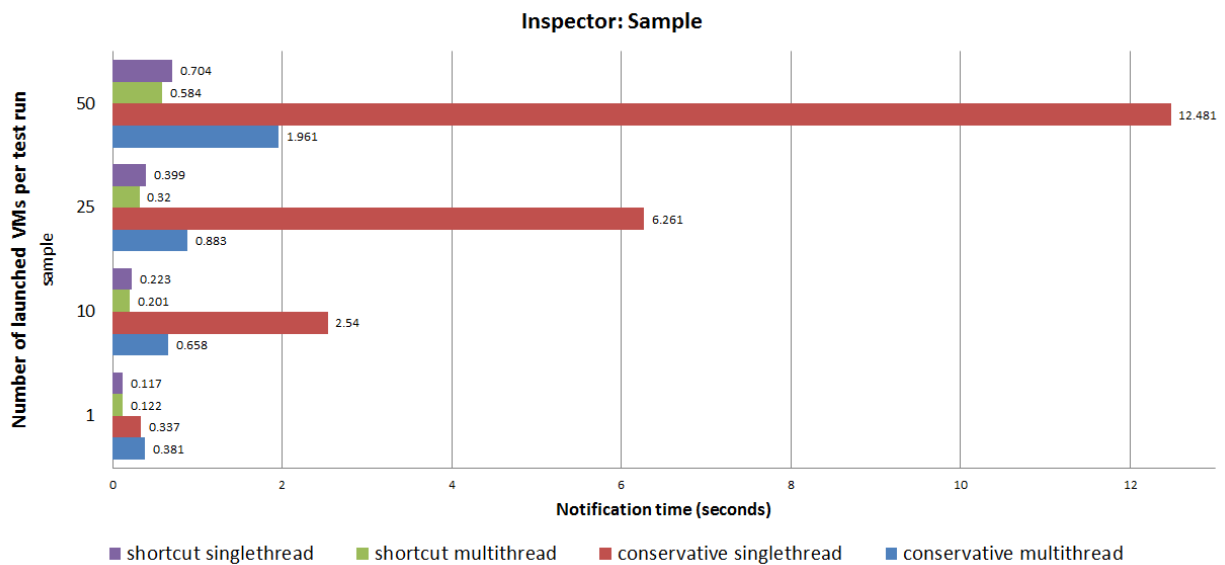
Fig. 3: Notification Time
